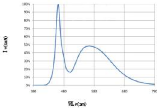
Fig.3 Relative Luminous Intensity vs. Wavelength
