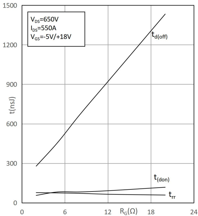
Fig.19 Switching Times vs. Gate Resistor( T_{vj}=150^{\circ}\text{C} ) 图19: 开关时间与门极电阻关系( T_{vj}=150^{\circ}\text{C} )
