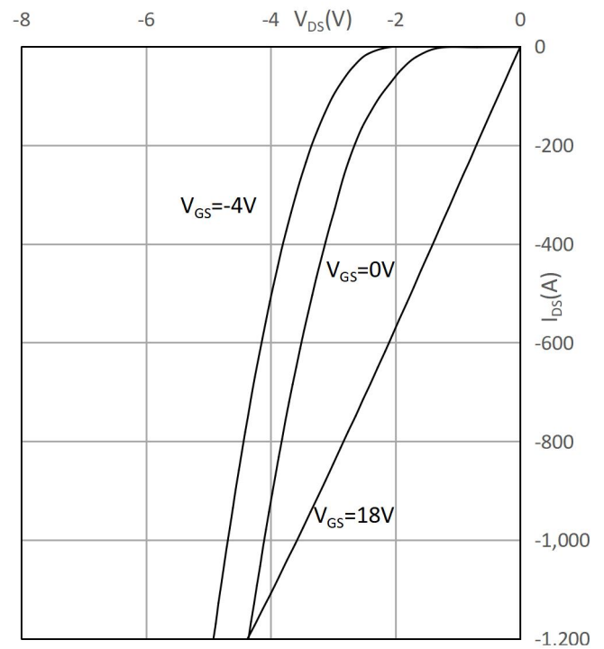
Fig.8 3rd Quadrant Characteristics( T_{vj}=150^{\circ}\text{C} )
