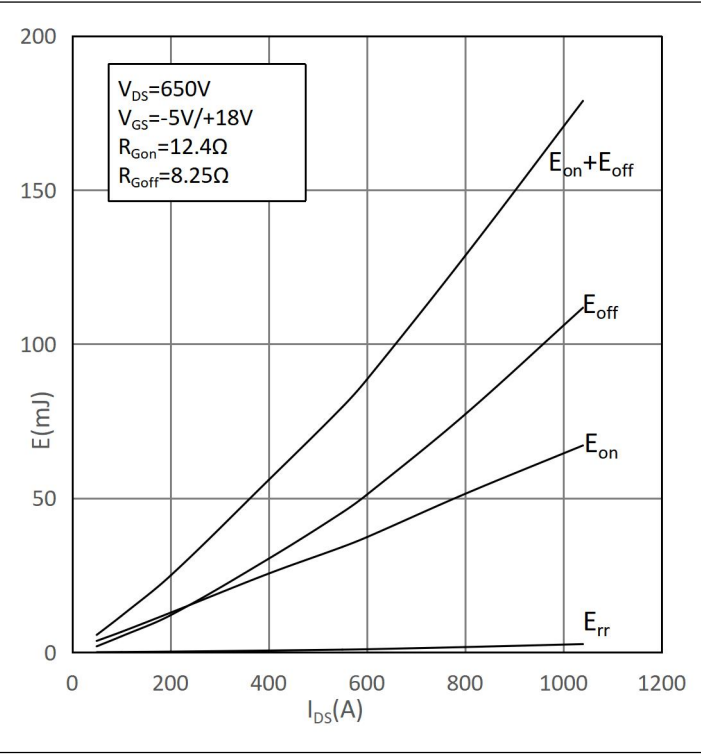
Fig.12 Switching Loss vs. Drain Current ( T_{vj}=175^{\circ}\text{C} ) 图12: 开关损耗与漏极电流的关系( T_{vj}=175^{\circ}\text{C} )
