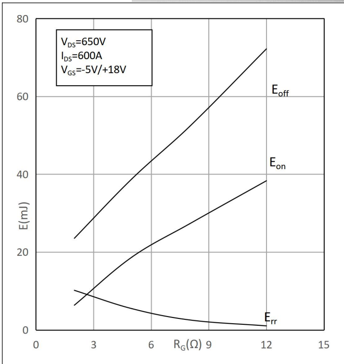
Fig.17 Switching Loss vs. Gate Resistor( T_{vj}=175^{\circ}\text{C} ) 图17: 开关损耗与门极电阻关系( T_{vj}=175^{\circ}\text{C} )
