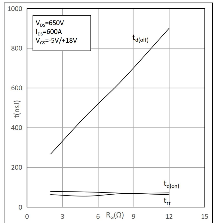
Fig.20 Switching Times vs. Gate Resistor( T_{vj}=175^{\circ}\text{C} ) 图20: 开关时间与门极电阻关系( T_{vj}=175^{\circ}\text{C} )
