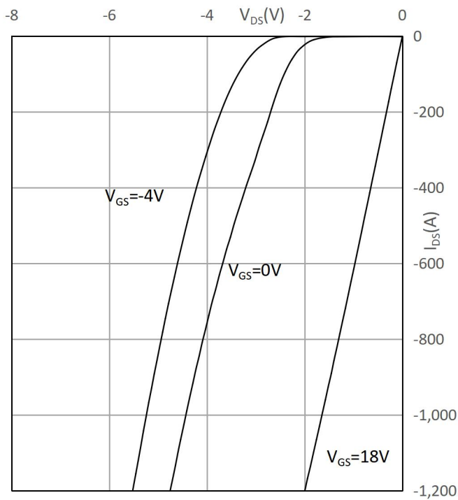
Fig.7 3rd Quadrant Characteristics( T_{vj}=25^{\circ}\text{C} )
