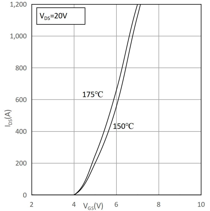
Fig.6 Typ. Transfer Characteristics
