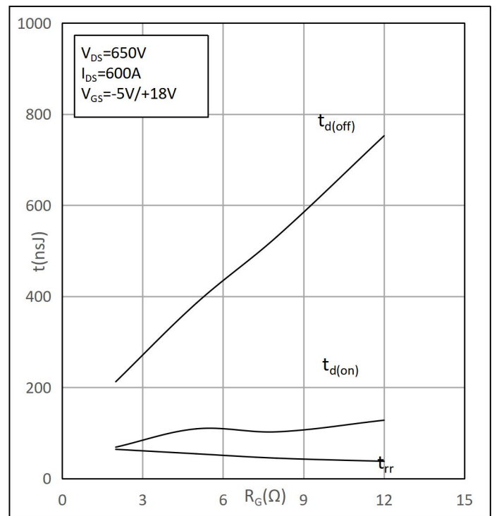
Fig.18 Switching Times vs. Gate Resistor ( T_{vj}=25^{\circ}\text{C} ) 图18: 开关时间与门极电阻关系( T_{vj}=25^{\circ}\text{C} )
