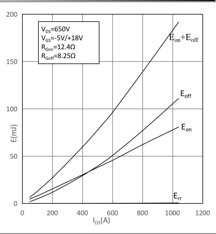
Fig.10: Switching Loss vs. Drain Current( T_{vj}=25^{\circ}\text{C} ) 图10: 开关损耗与漏极电流的关系( T_{vj}=25^{\circ}\text{C} )
