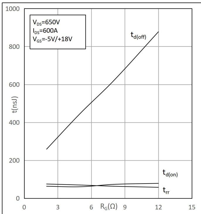
Fig.19 Switching Times vs. Gate Resistor( T_{vj}=150^{\circ}\text{C} ) 图19: 开关时间与门极电阻关系( T_{vj}=150^{\circ}\text{C} )
