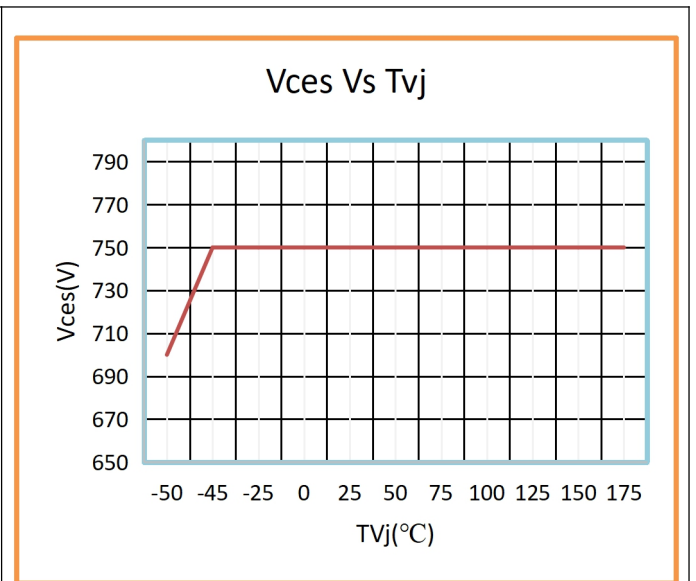
Maximum allowed collector-emitter voltage Ices=1mA for T_{vj} \leq 25^\circ\text{C} , Ices=30mA for T_{vj} > 25^\circ\text{C}
