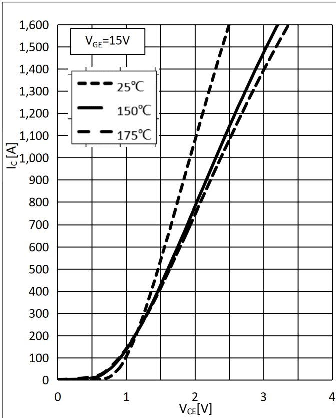
Fig.1: On-state Characteristics
