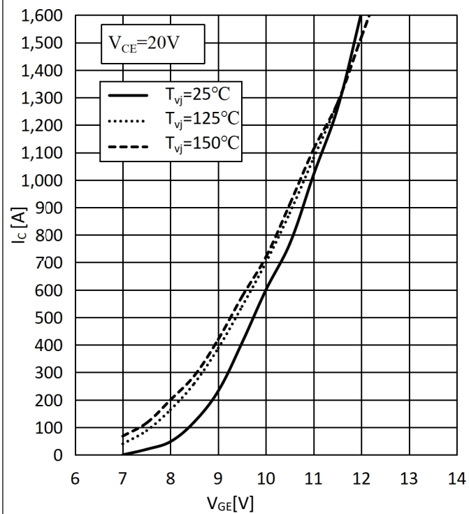
Fig.3: Transfer Characteristics
