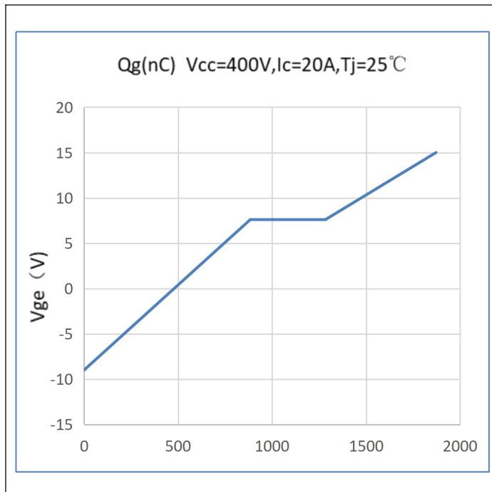
Fig. 15: Typ. Gate charge characteristic IGBT
