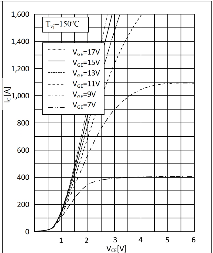
Vce[V] Fig.2: Output characteristics
