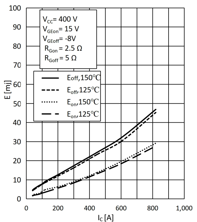
Fig.4: Switching Loss vs. Collector Current
