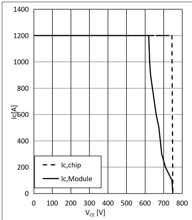
Fig. 11: Reverse Bias Safe Operating Area
