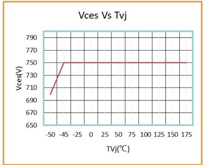
Maximum allowed collector-emitter voltage Ices=1mA for Tvj≤25°C, Ices=30mA for Tvj>25°C
