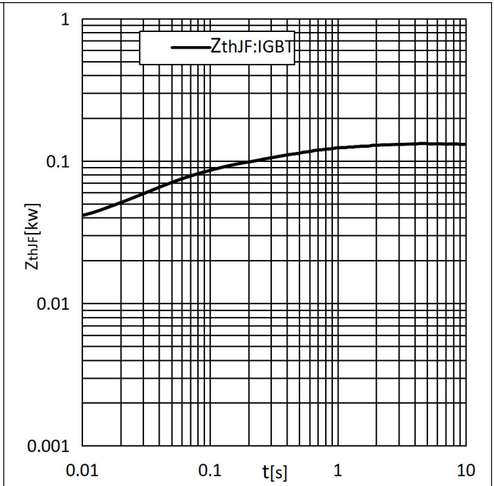
Fig.14: Typ. transient thermal impedance(IGBT) Z_{thJF} IGBT(K/W)
