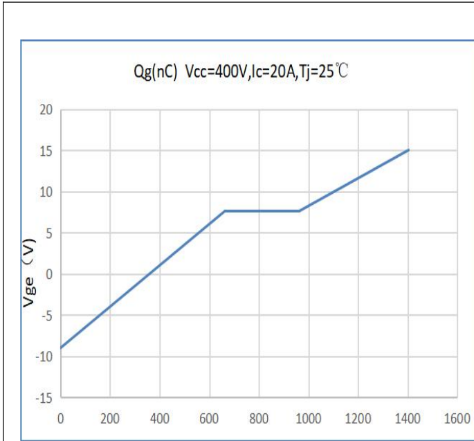
Fig. 15: Typ. Gate charge characteristic IGBT
