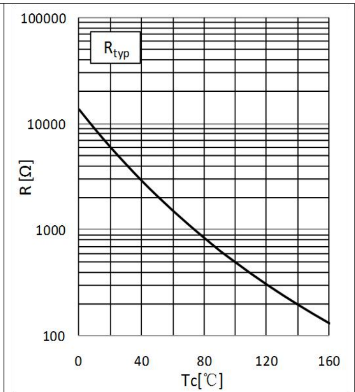
Fig.12:Typ. NTC-Temperature Characteristics
