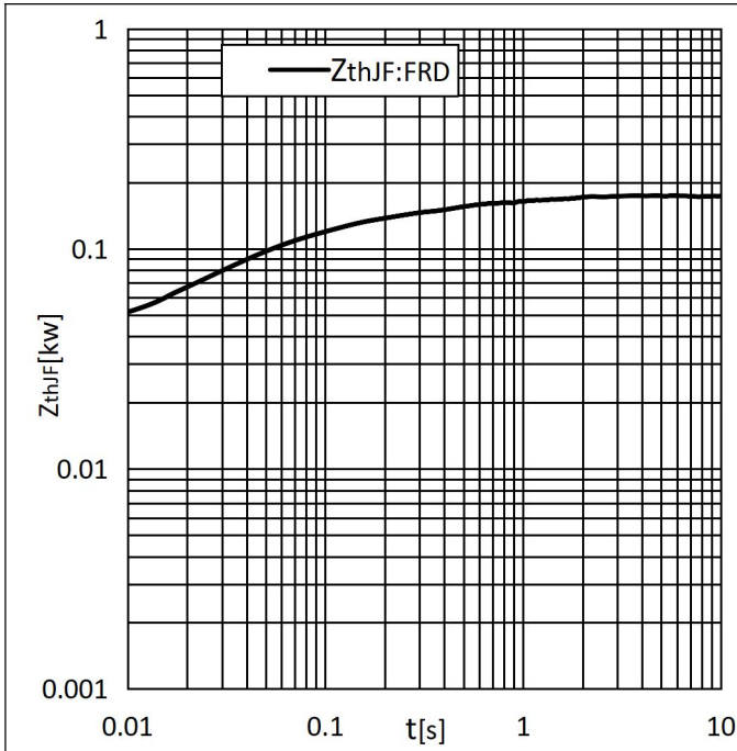
Fig.13: Typ. transient thermal impedance(FRD) Z_{thJF} FRD(K/W)
