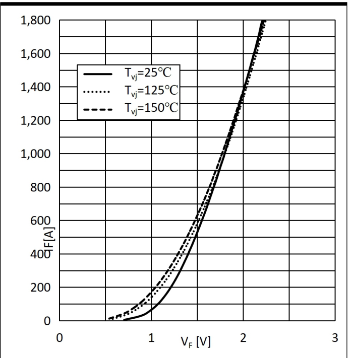
Fig.8: Forward characteristic 图8: 正向特性
