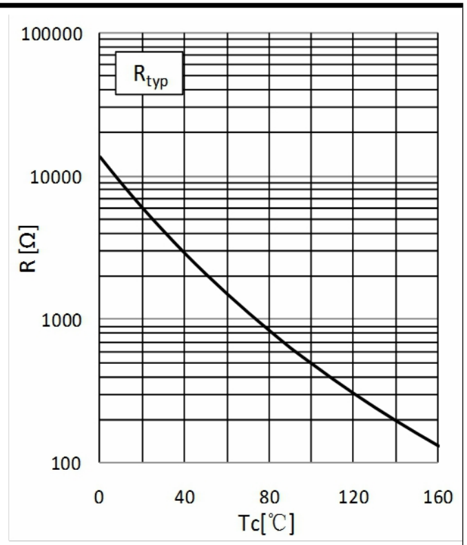
Fig. 12: Typ. NTC-Temperature Characteristics
