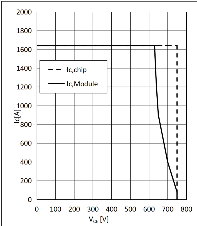
Fig. 11: Reverse Bias Safe Operating Area
