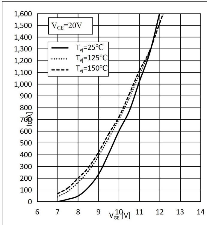
Fig.3: Transfer Characteristics
