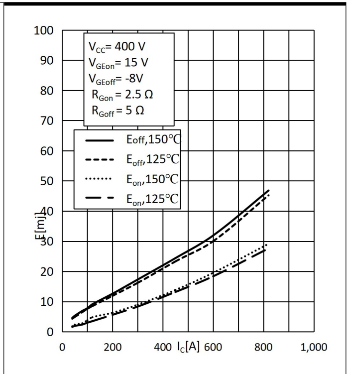
Fig.4: Switching Loss vs. Collector Current
