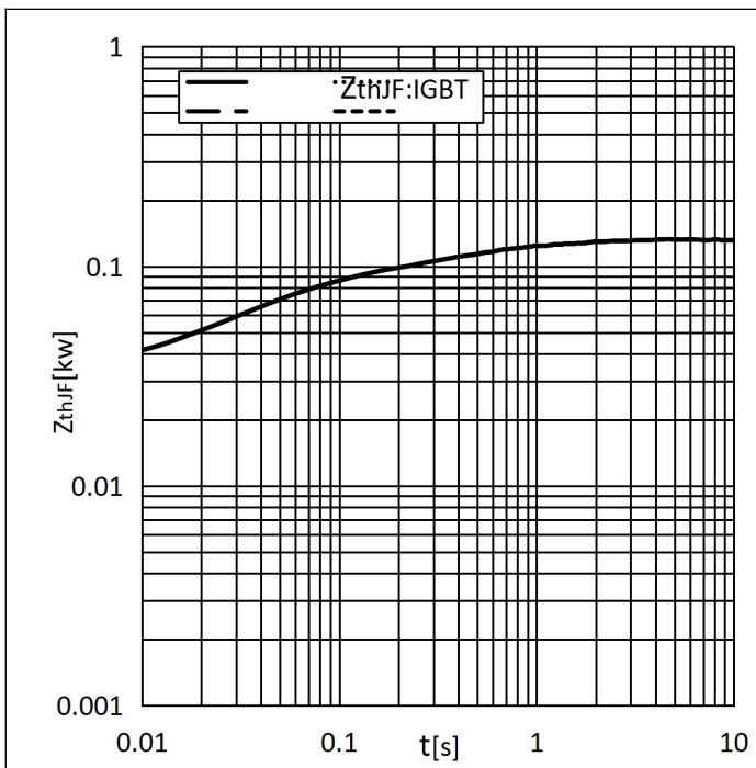
Fig. 13: Typ. transient thermal impedance(IGBT) Z_{thJF} IGBT(K/W)
