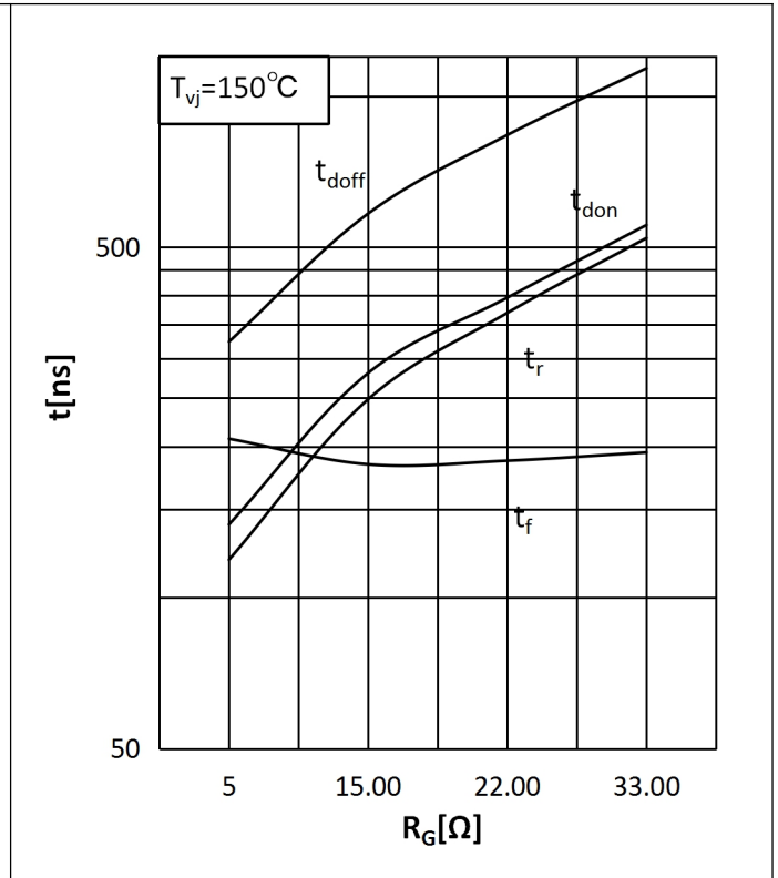
Fig.6: Switching Times vs. Gate Resistor
