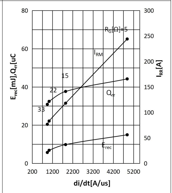
Fig.8: Reverse recovery characteristics vs. di/dt
