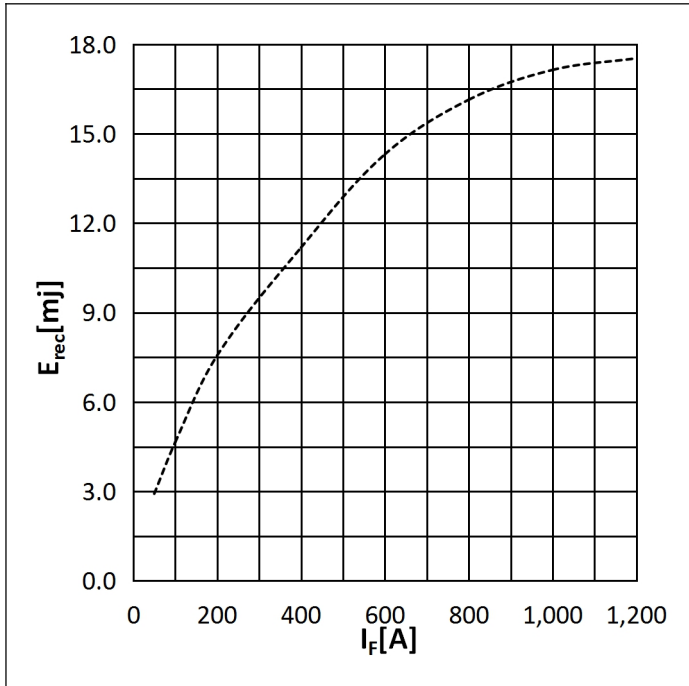
Fig.9: Reverse recovery Energy
