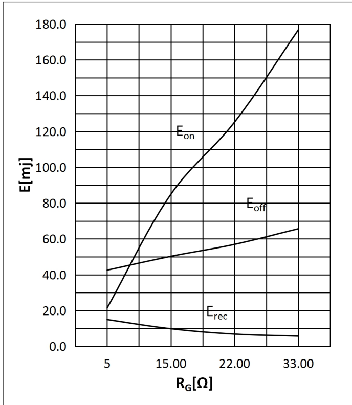
Fig.5: Switching Loss vs. Gate Resistor
