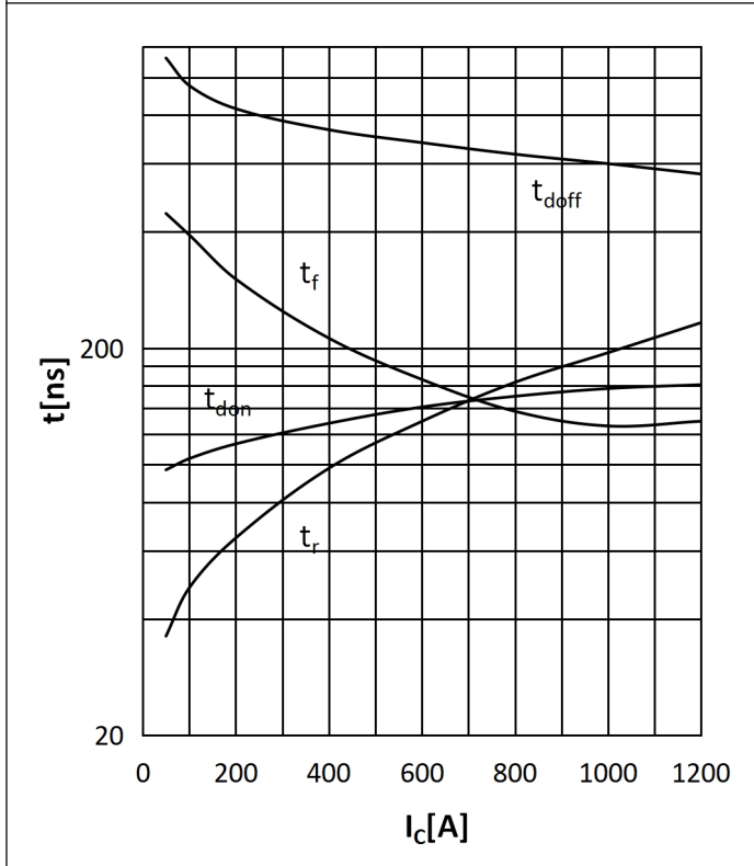
Fig.7: Switching Times vs. I_c
