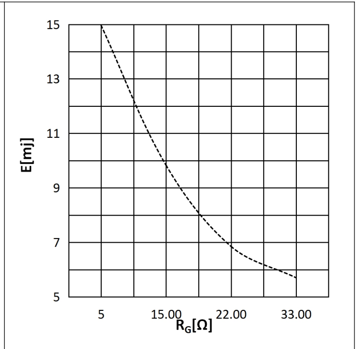
Fig.10: Reverse recovery Energy vs. Gate Resistor
