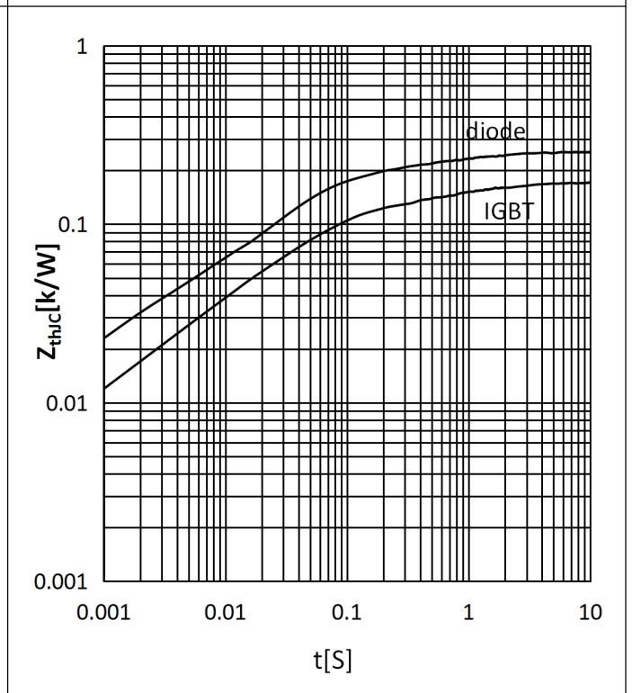
Fig.11: Typ. transient thermal impedance
