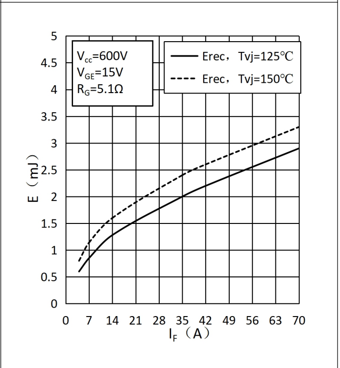
Fig.8 Typ. Switching Losses of Diode-Inverter
