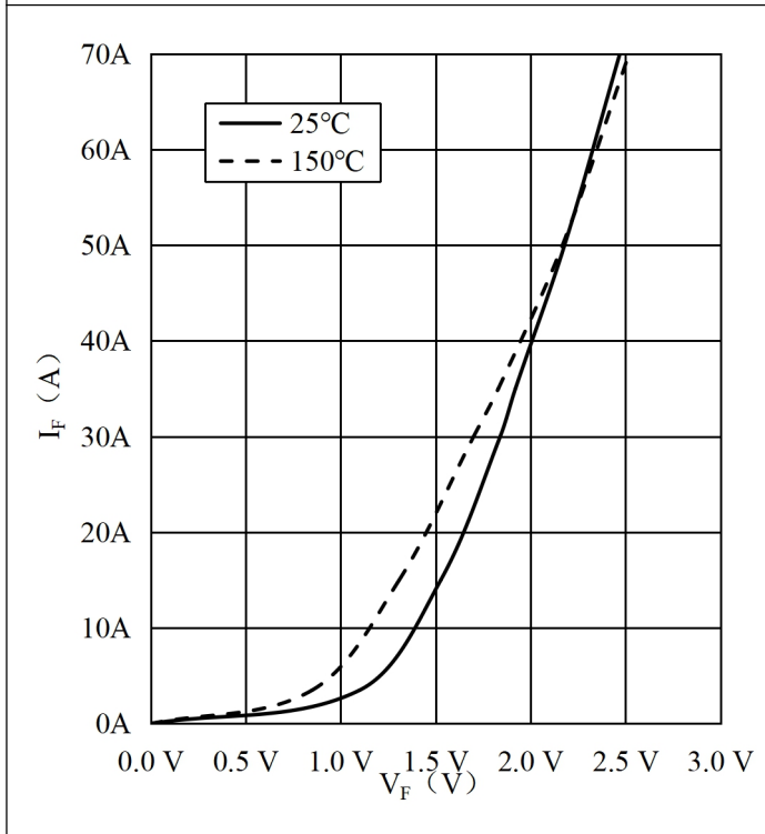
Fig.7 Typ. Forward Characteristics of Diode-Inverter
