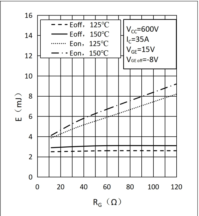
Fig.6 Switching Loss of IGBT vs. Gate Resistor - Inverter
