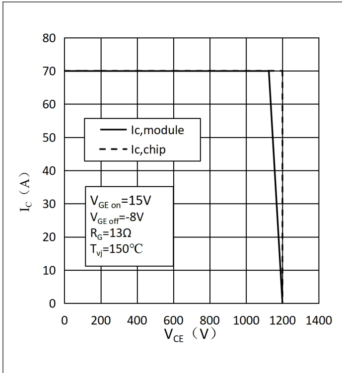
Fig.5 Reverse Bias Safe Operating Area (RBSOA) -Inverter
