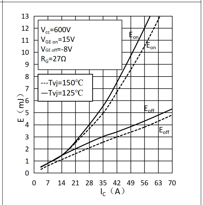
Fig.4 Switching Loss vs. Collector Current-Inverter 图 4 开关损耗和集电极电流-逆变器
