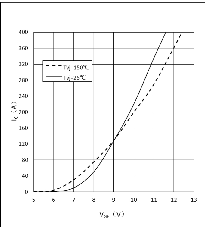
Fig.2 Typ. Transfer Characteristics-Inverter
