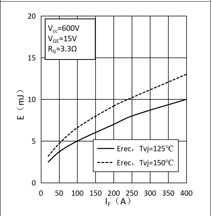
Fig.8 Typ. Switching Losses of Diode-Inverter 图 8 二极管开关损耗-逆变器
